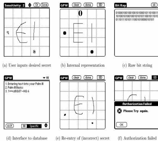
A graphical password scheme proposed by Jansen, et al
