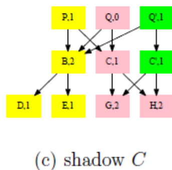
Figure 5: Inserting a key into node H of tree T_q . The path from Q to H includes nodes \{Q, C, H\} , these are all COWed. Sharing is broken for nodes C and H; the ref-count for C is decremented.
