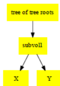
Figure 12: Upper level nodes stored in a backref cache.
