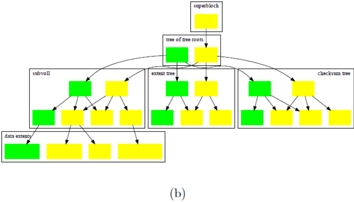
Figure 9: (a) A filesystem forest. (b) The changes that occur after modification; modified pages are colored green.
