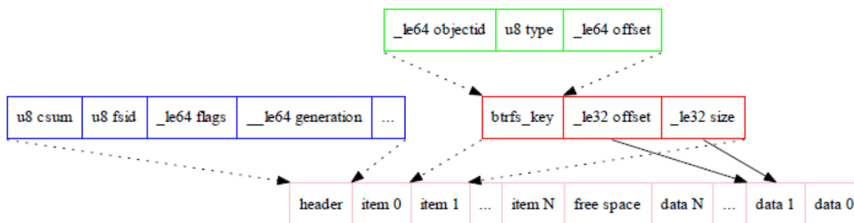
Figure 8: A detailed look at a generic leaf node holding keys and items.
