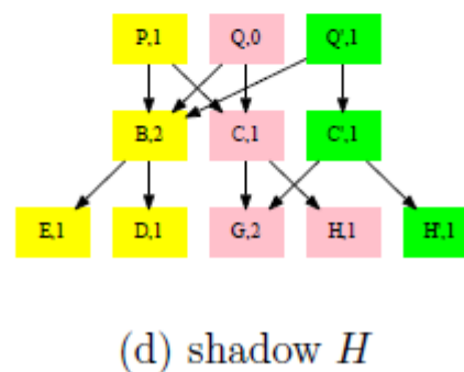
Figure 5: Inserting a key into node H of tree T_q . The path from Q to H includes nodes \{Q, C, H\} , these are all COWed. Sharing is broken for nodes C and H; the ref-count for C is decremented.
