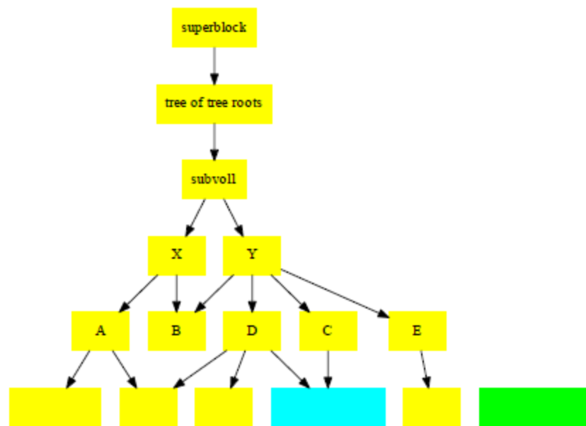
Figure 11: Do a range lookup in the extent tree, find all the extents located in the chunk. Copy all the live extents to new locations.
