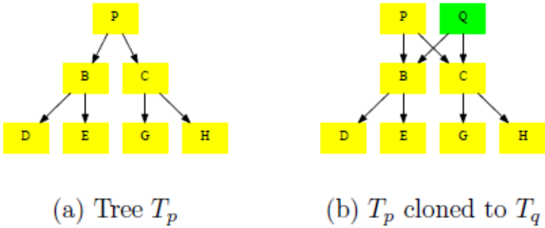
Figure 3: Cloning tree T_p . A new root Q is created, initially pointing to the same blocks as the original root P . As modifications will be applied, the trees will diverge.
