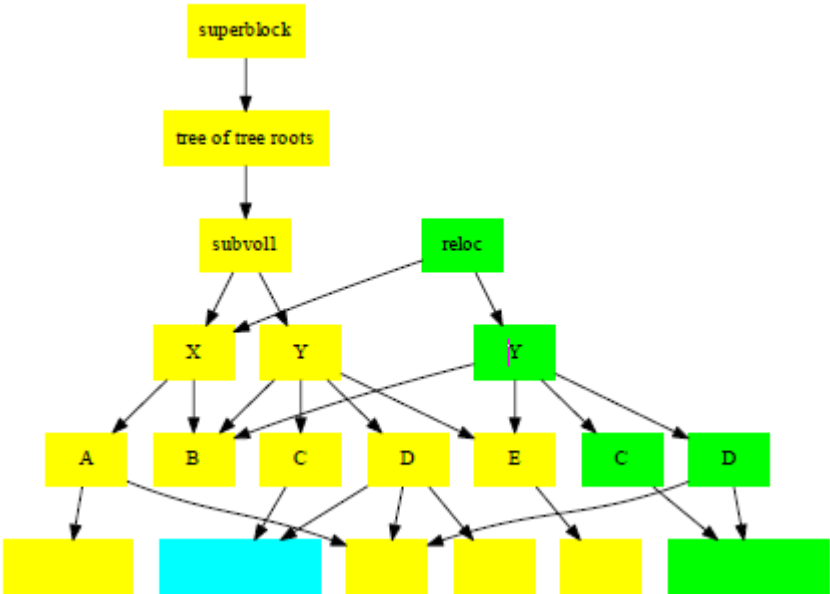
Figure 14: Fix references in the reloc tree using COW.
