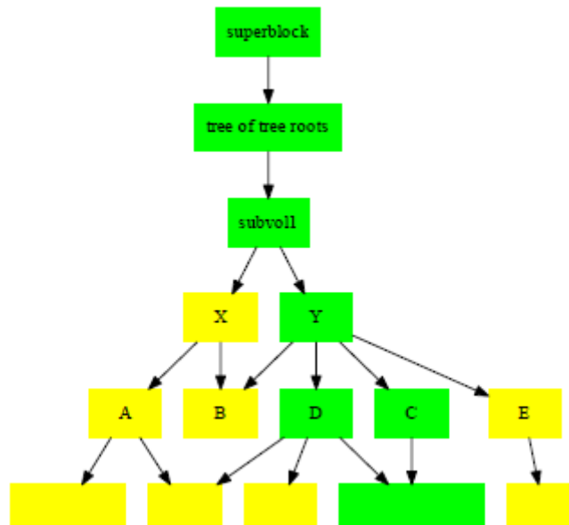
Figure 15: Merge reloc trees with corresponding fs trees, then drop the reloc trees.
