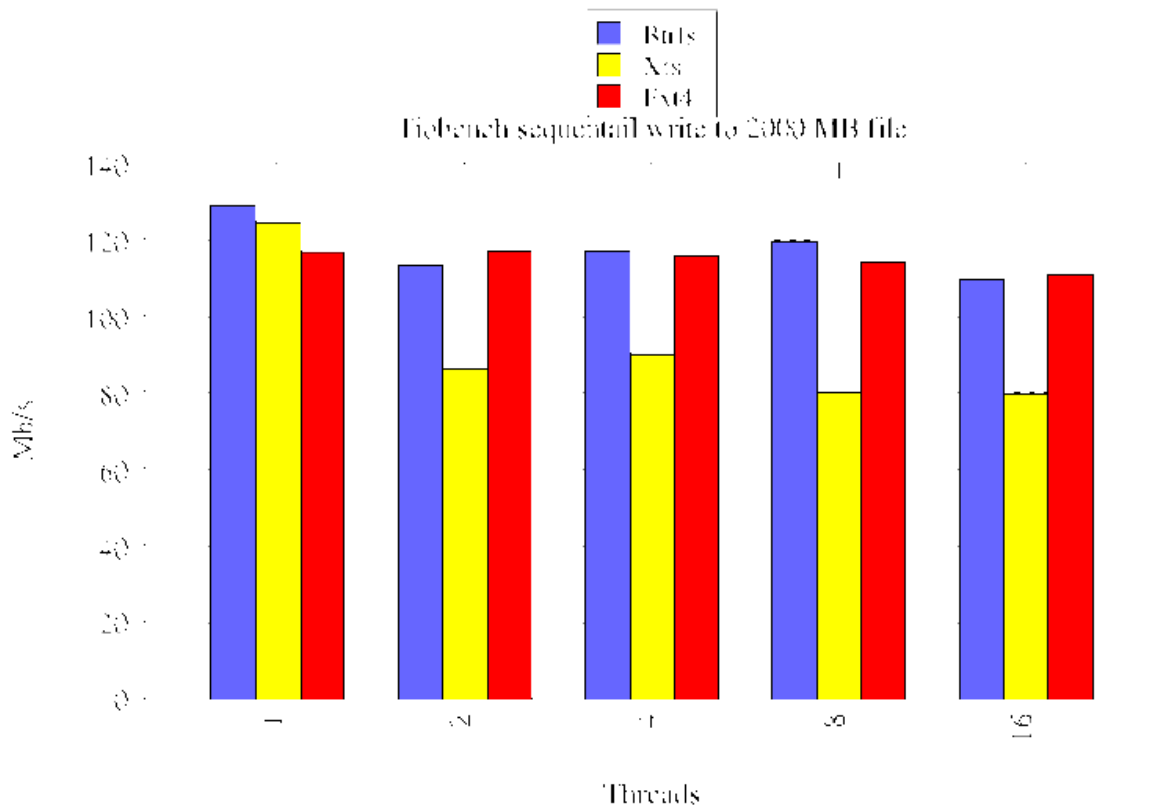
Figure 19: TIO benchmark, sequential.
