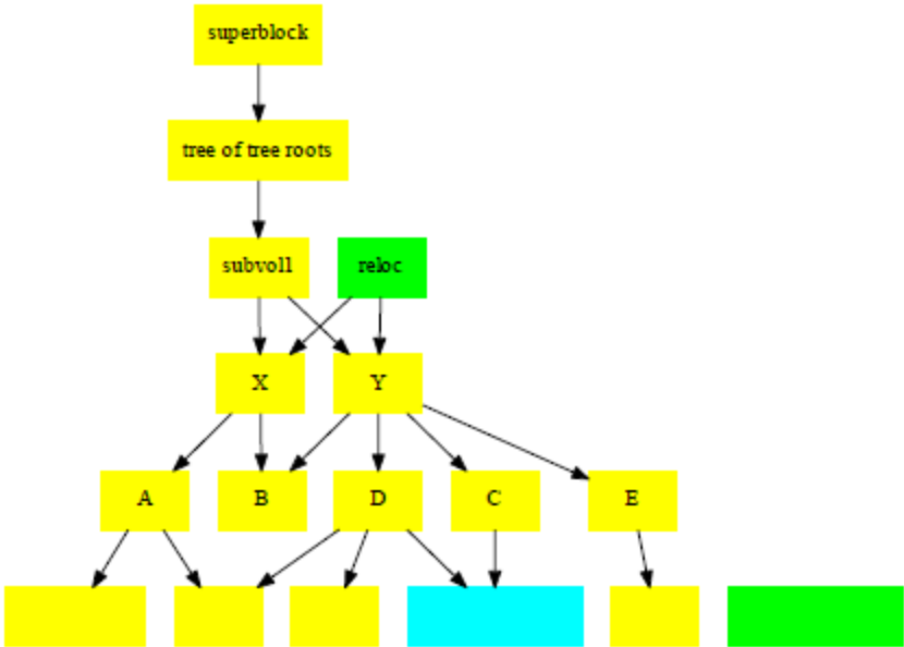
Figure 13: Reloc trees. In this example, sub-volume1 is cloned. Changes can be made to the clone.
