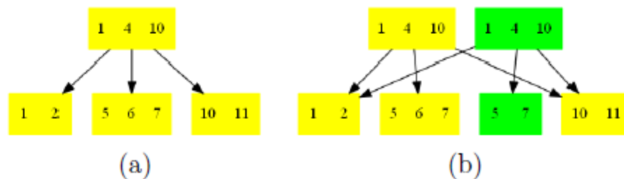
Figure 2: (a) A basic tree (b) Deleting key 6.
