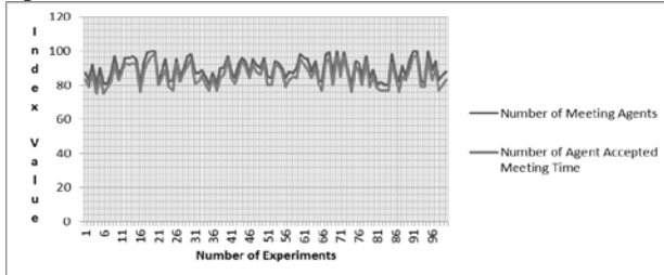
Fig. 5 Number of Meeting agents Vs. Agents accepted meeting time
