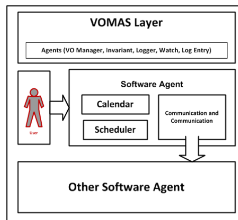
Fig. 4 Virtual Overlay Multi-agent System
