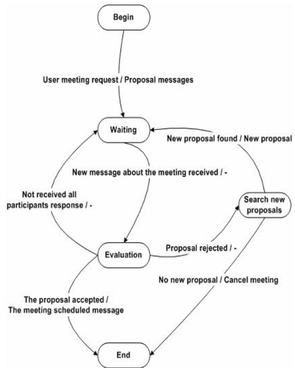
Fig. 2 State Transition of agent during scheduling
