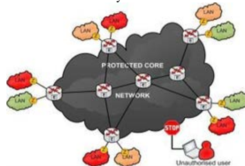
Fig.1. Military Networks
